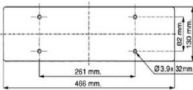
VISTA FRONTALE / FRONT VIEW
